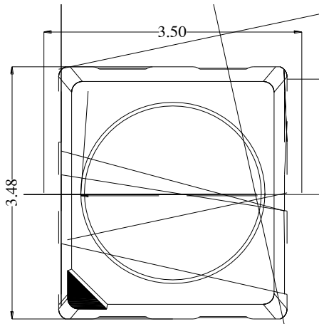
Fig.1-1 Top View
