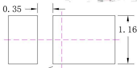
Fig.1-5 Soldering patterns
