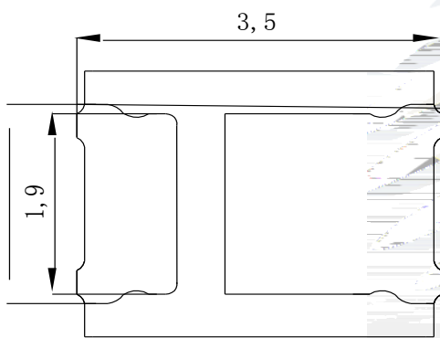
Fig.1-3 Bottom view
