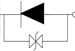
Fig.1-4 Polarity
