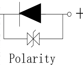
Fig.1-4 Polarity
