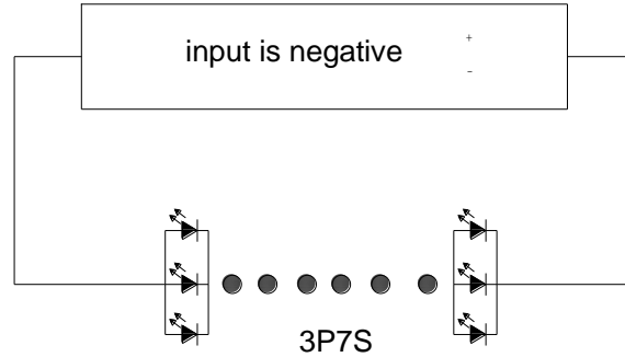
Fig.2-2 Product connection
