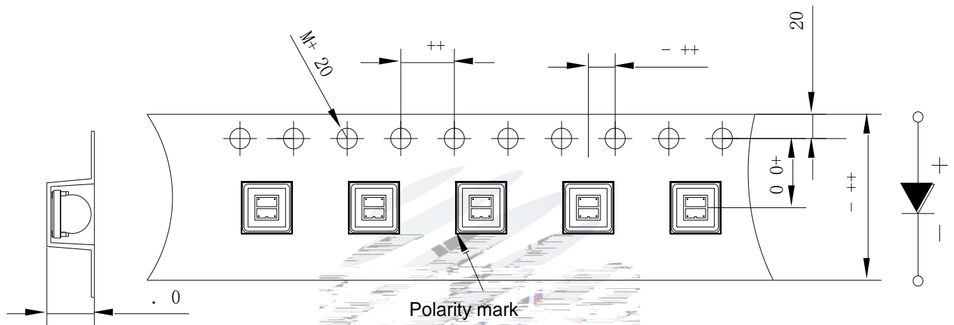
Fig.2-1 Carrier-Tape Dimension
