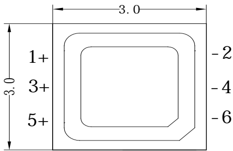
Fig 1-1 Top view
