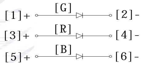
Fig 1-4 Polarity
