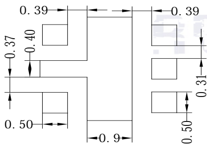
Fig 1-5 Soldering patterns
