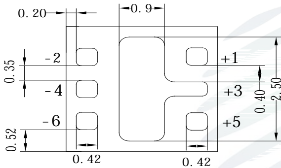
Fig 1-3 Bottom view
