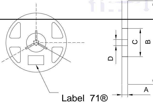
Fig.2-2 Reel Dimension
