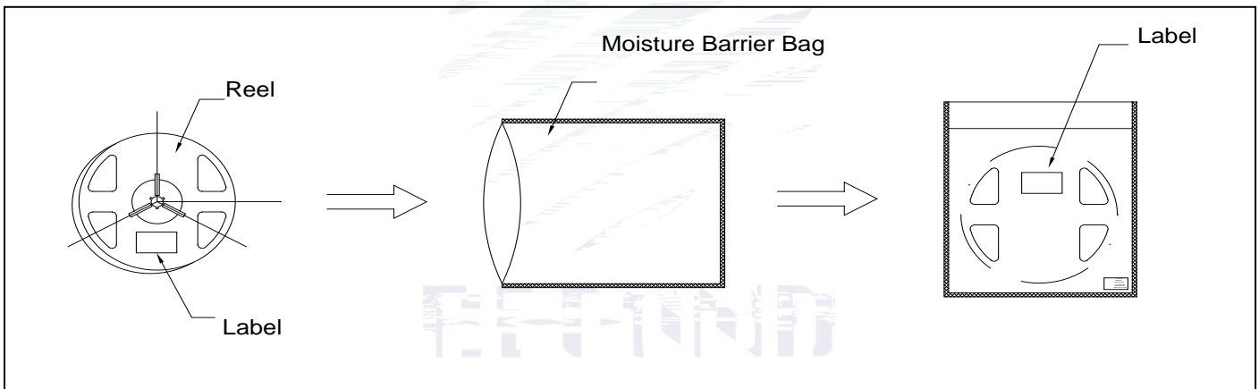
Fig.2-4Moisture Resistant Packing
